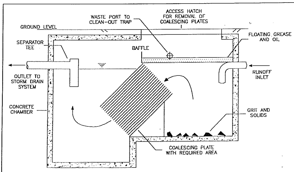
Figure 4.5 Coalescing Plate Oil-Water Separator
