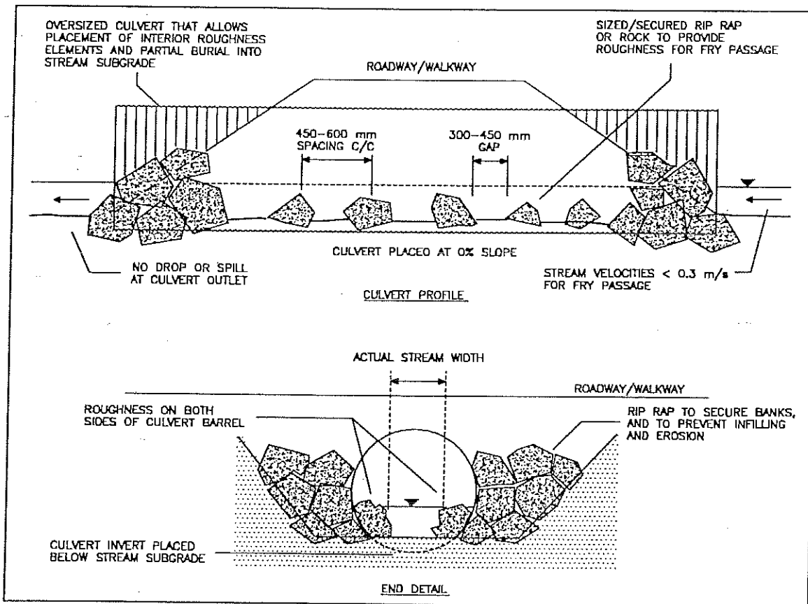
Figure 6.3 Culvert Installation for a Small Creek with Provision for Fry Passage
