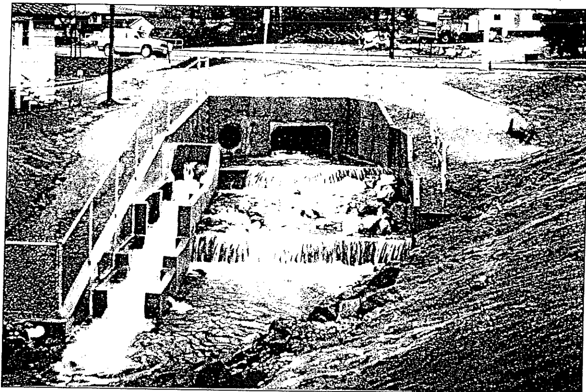
Figure 6.2 Culvert Providing Upstream Fish Passage
