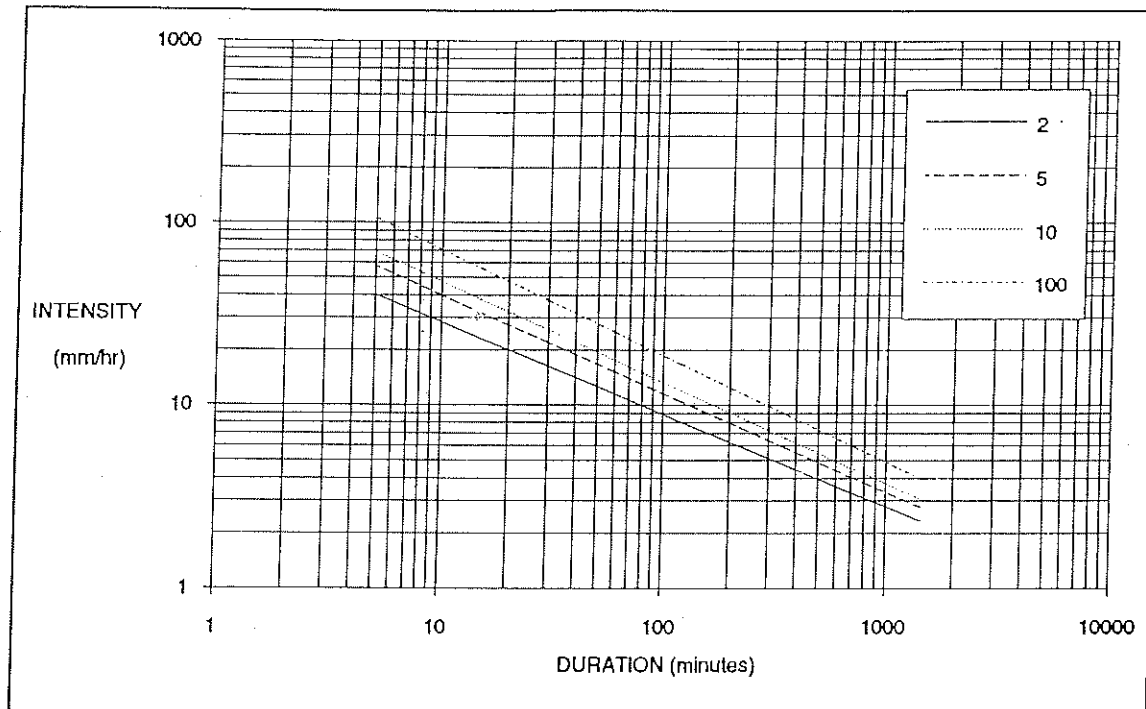
Figure 8.5 Land Development Example Site IDF Curves
