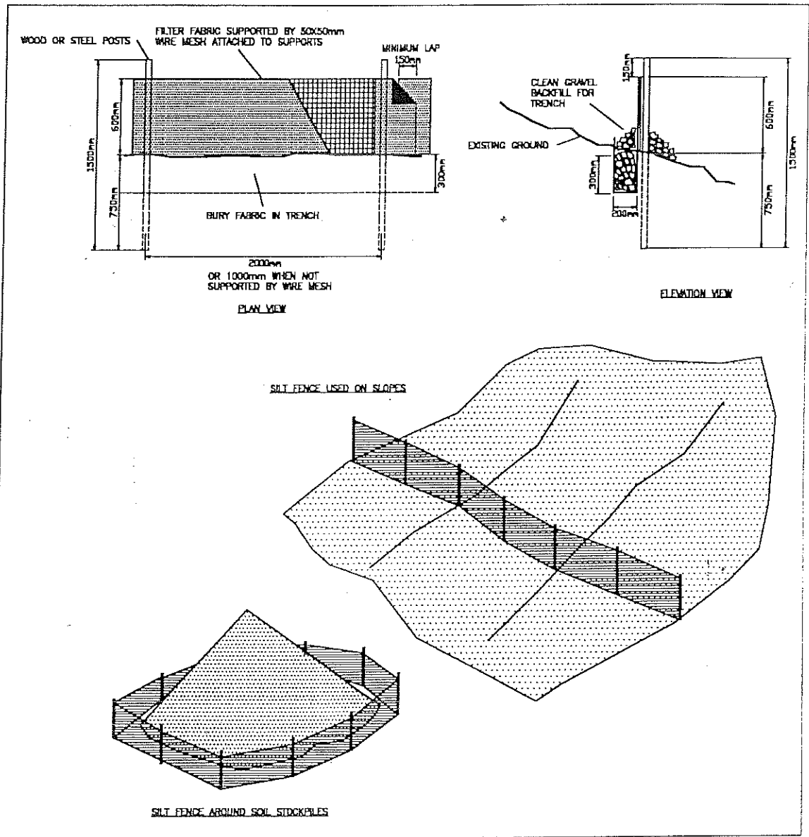
Figure 3.3 Typical Silt Fence Construction and Applications
